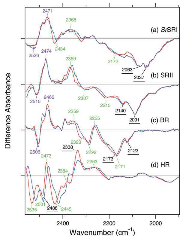
FIGURE 5: \text{SrSRI}_K minus \text{SrSRI} (a) difference infrared spectra measured at pH 7.0 in the 2560 – 1900\text{ cm}^{-1} region. The samples were hydrated with \text{D}_2\text{O} (red line) and with \text{D}_2^{18}\text{O} (blue line). Underline, green label, and purple label correspond to C=N stretching vibration, vibration of water molecules, and vibration of threonine residue, respectively. The \text{SRII}_K minus \text{SRII} (b), \text{BR}_K minus BR (c), and \text{HR}_K minus HR (d) difference FTIR spectra are reproduced from refs 34, 35, and 36, respectively, for comparison. One division of y axis corresponds to 0.0012 absorbance units.
