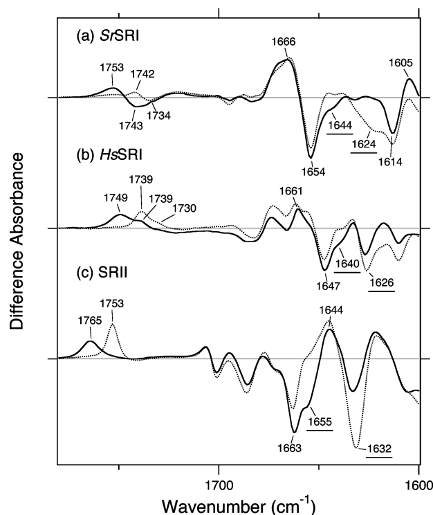
FIGURE 7: SrSRI_M minus SrSRI (a) difference infrared spectra measured at 260 K at pH 7.0 in the 1780–1600 cm^{-1} region. The samples were hydrated with H_2O (—) or D_2O (····). Underlined values corresponds to C=N stretching vibration. The HsSRI_M minus HsSRI (b) and SRII_M minus SRII (c) difference FTIR spectra are reproduced from refs 32 and 39, respectively, for comparison. One division of y axis corresponds to 0.01 absorbance units.
